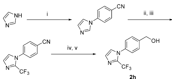
Scheme 4. (i) 4-fluorobenzonitrile, \text{K}_2\text{CO}_3 , DMSO; (ii) n\text{-BuLi} , THF; (iii) \text{TMS-CF}_3 , \text{CuI} , \text{KF} , DMF, 1-methyl-2-pyrrolidone; (iv) Dibal-H, \text{CH}_2\text{Cl}_2 ; (v) \text{NaBH}_4 , EtOH.
