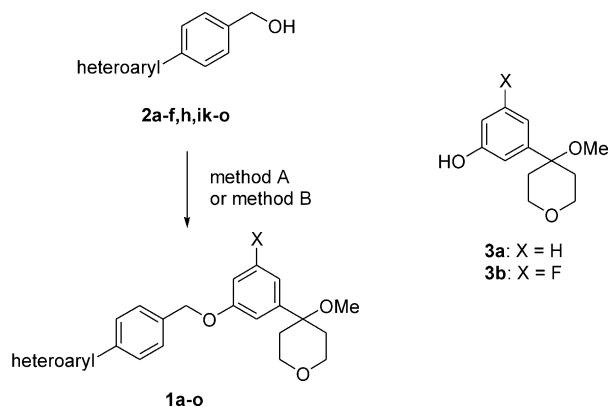
Scheme 1. Method A: 3a or 3b , DEAD, TEA, THF; Method B: (i) \text{SOCl}_2 ; (ii) 3b , \text{K}_2\text{CO}_3 , DMF. Generic groups presented as heteroaryl are defined in Table 1.
