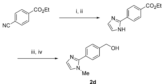
Scheme 3. (i) \text{NH}_2\text{CH}_2\text{CH}_2\text{NH}_3^+ 4\text{-MePhSO}_3^- ; (ii) \text{BaMnO}_4 ; (iii) \text{MeOCOCOMe} , \text{K}_2\text{CO}_3 ; (iv) Dibal-H, \text{CH}_2\text{Cl}_2 .
