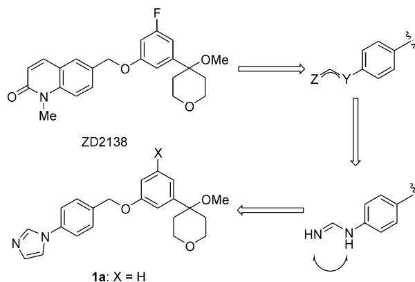
Scheme 5. Evolution of imidazole 5-LOI from ZD2138.
