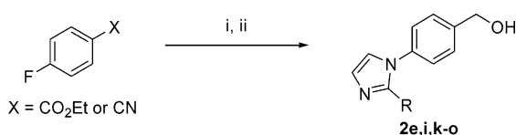
Scheme 2. (i) 2-R-1H-imidazole, base; (ii) Dibal-H, THF or Dibal-H, \text{CH}_2\text{Cl}_2 then \text{NaBH}_4 , EtOH.
